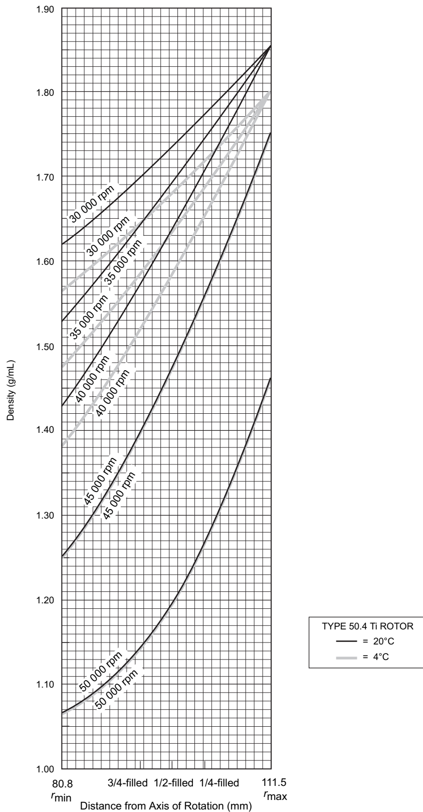
Figure 2 CsCl Gradients at Equilibrium for the Type 50.4 Ti Rotor (Outer Row). Centrifugation of homogeneous CsCl solutions at the maximum allowable speeds (from Figure 1 ) results in gradients presented here.
