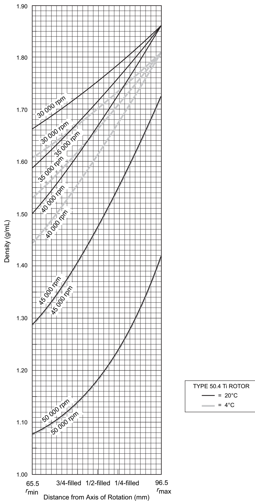
Figure 4 CsCl Gradients at Equilibrium for the Type 50.4 Ti Rotor (Inner Row). Centrifugation of homogeneous CsCl solutions at the maximum allowable speeds (from Figure 1 ) results in gradients presented here.
